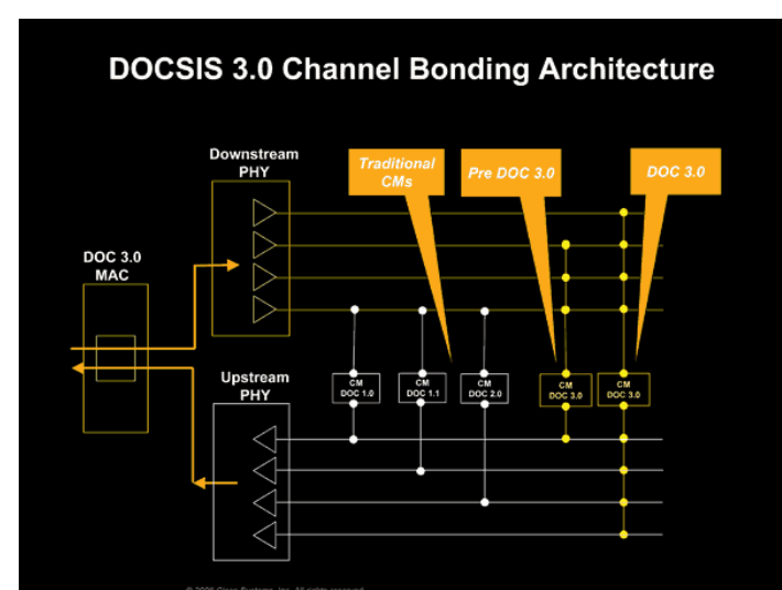
FIGURE 1: DOCSIS 3.0 channel bonding
